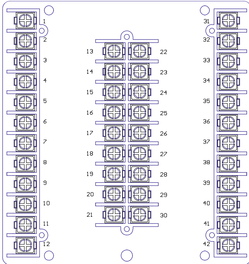
Rear view of LKE-DPR-T-201
