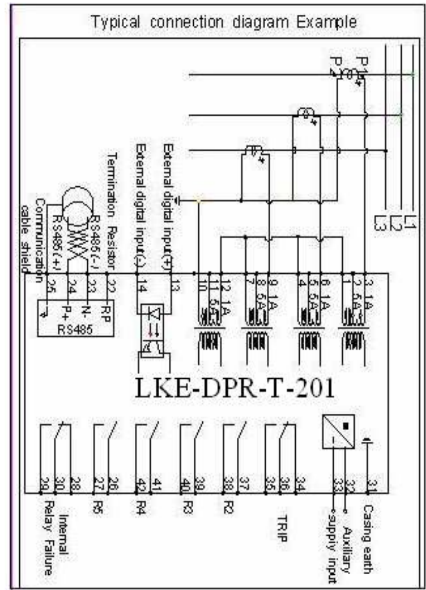
Example 1: Typical connection diagram Example
